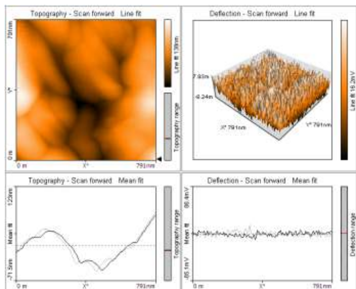
Figure 7 AFM image of Cymbopogon citratus mediated synthesized silver nanoparticles
