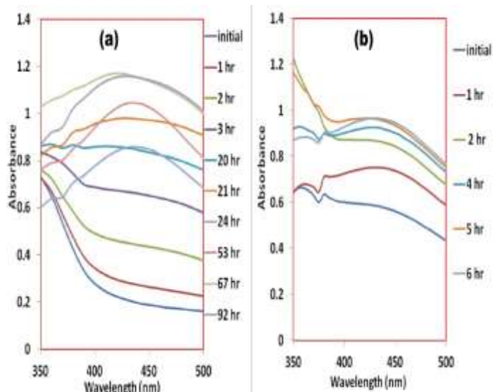
Figure 3 UV-Vis spectra of nanoparticles (a) unboiled sample (b) 2 minutes microwave heated the sample
