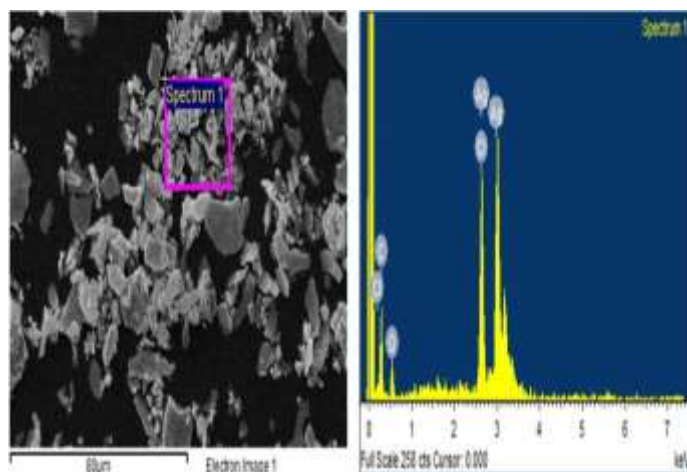
Figure 6 (b) EDAX analysis of silver nanoparticles
