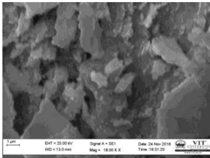
Figure 6 (a) SEM image of the silver nanoparticles
