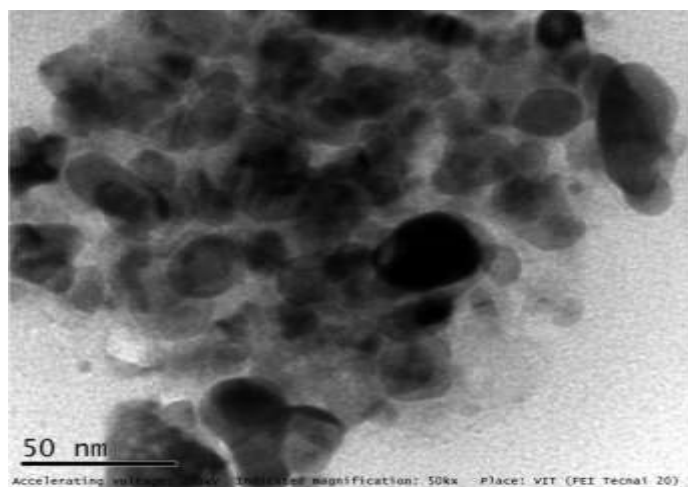
Figure 8 TEM Image of silver nanoparticles
