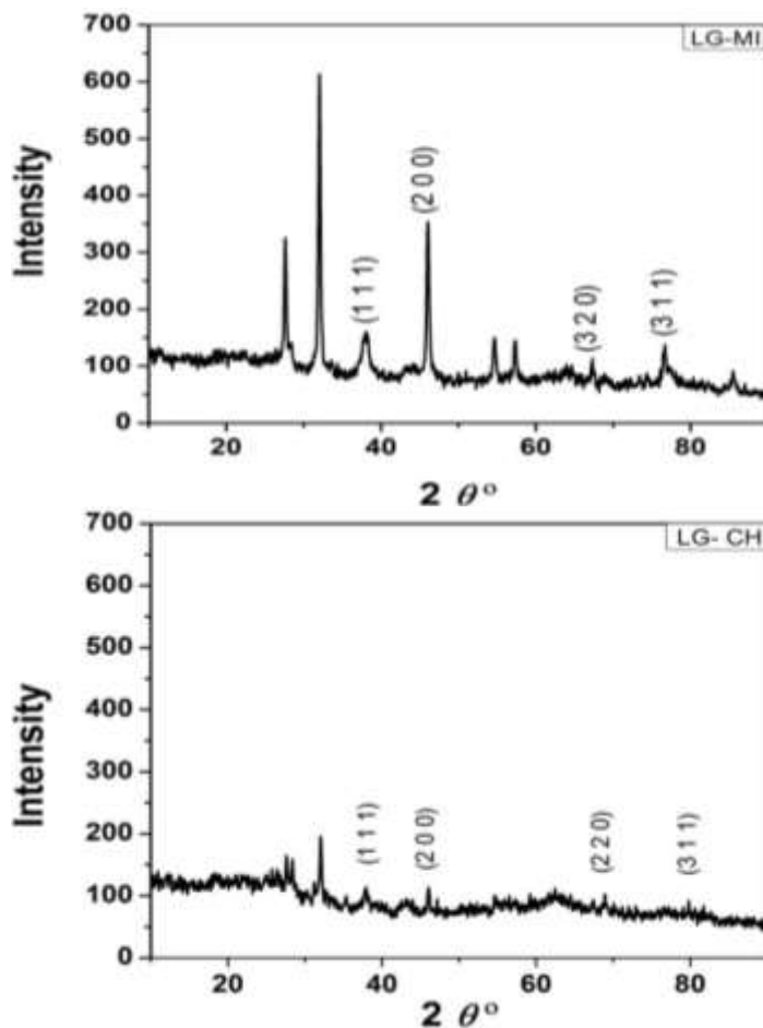
Figure 4 (a) XRD spectra of 2 minutes MI silver nanoparticles (b) XRD spectra of the conventionally heated silver nanoparticles
