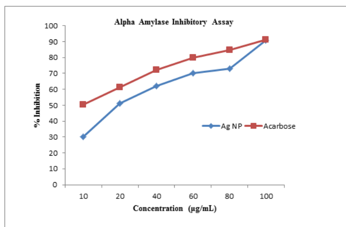
Figure 9 Alpha-amylase inhibitory assays of silver nanoparticles
