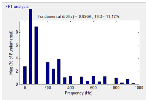
Figure 11. Voltage THD Value of sag due to loads before compensation.
