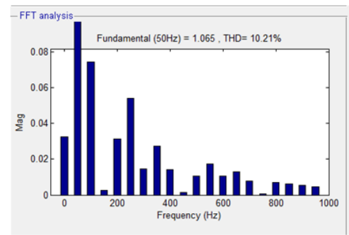
Figure 32. Voltage THD Value of Swell due to loads before compensation.
