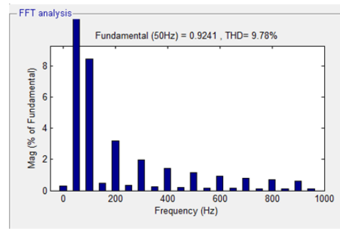
Figure 13. Voltage THD Value of unbalance before compensation.
