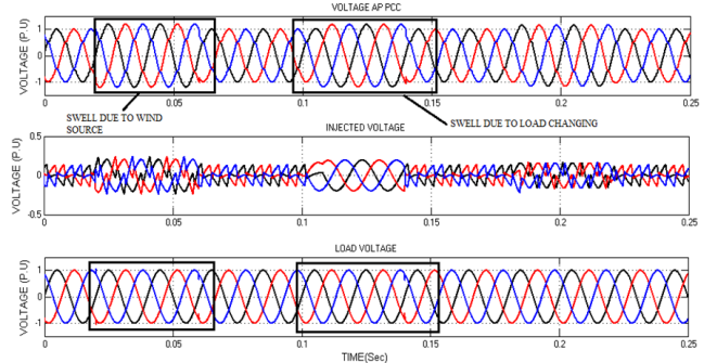
Figure 15. PCC voltage with swell, injected voltage, load voltage.
