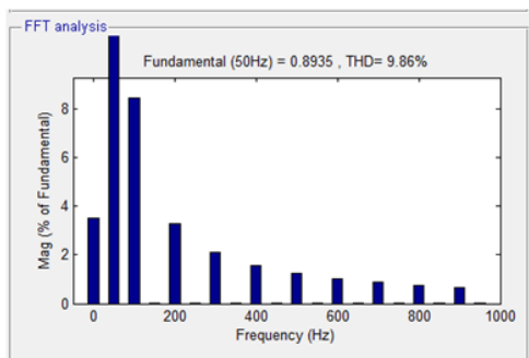
Figure 23. Voltage THD Value of Sag from wind source before compensation.
