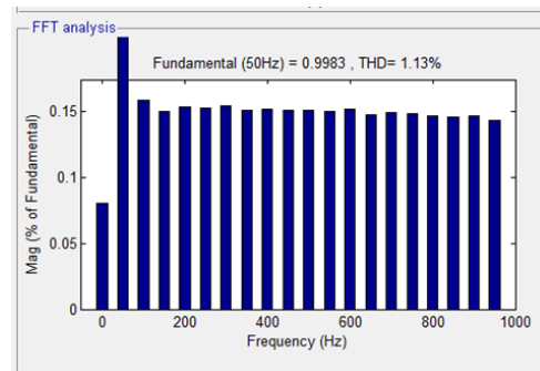
Figure 14. Voltage THD Value of unbalance after Compensation.
