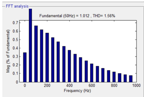
Figure 28. Voltage THD Value of unbalance after compensation.
