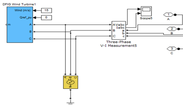
Figure 5. Simulink diagram of the DFIG.
