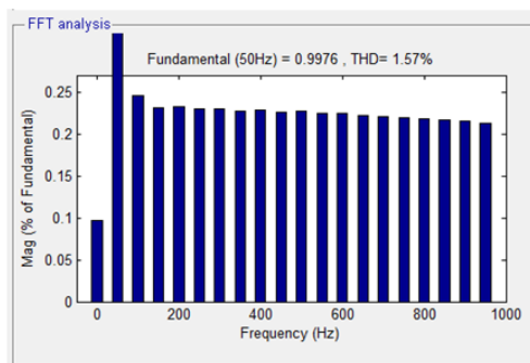
Figure 10. Voltage THD Value of Sag from wind source after compensation.
