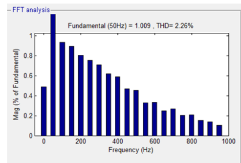
Figure 26. Voltage THD Value of sag due to loads after compensation.
