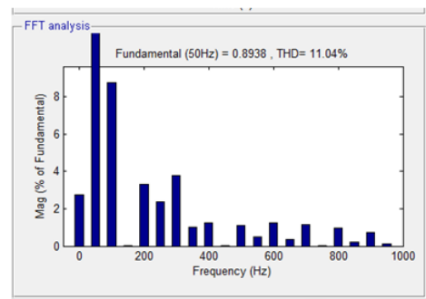
Figure 25. Voltage THD Value of sag due to loads before compensation.
