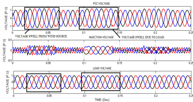
Figure 29. PCC voltage with swell, injected voltage, load voltage.
