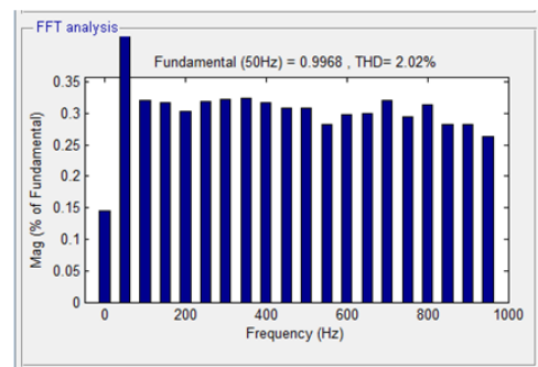
Figure 12. Voltage THD Value of sag due to loads after compensation.
