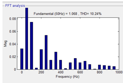
Figure 16. Voltage THD Value of Swell from wind source before compensation.
