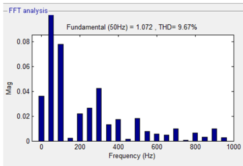
Figure 18. Voltage THD Value of Swell due to loads before compensation.
