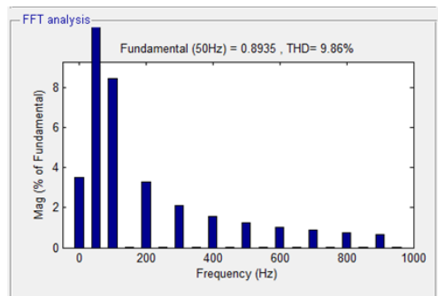
Figure 30. Voltage THD Value of Swell from wind source before compensation.
