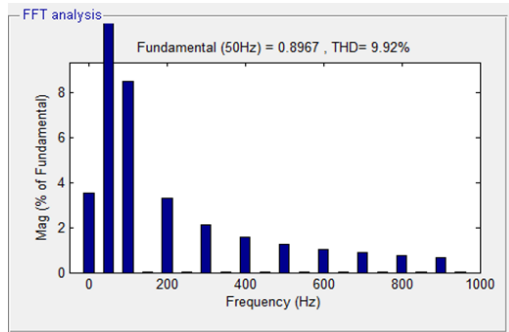
Figure 9. Voltage THD Value of Sag from wind source before compensation.
