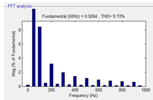
Figure 27. Voltage THD Value of unbalance before compensation.
