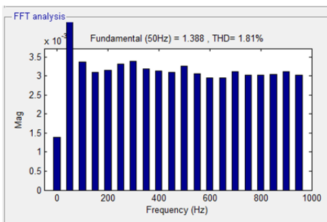
Figure 19. Voltage THD Value of Swell due to loads after compensation.
