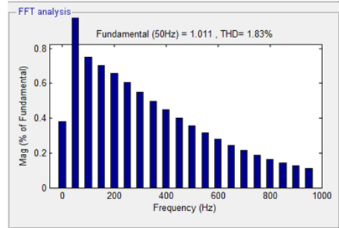
Figure 24. Voltage THD Value of Sag from wind source after compensation.
