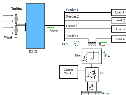
Figure 1. DVR with WECS.
