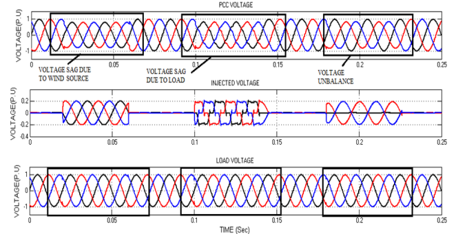
Figure 8. PCC Voltage with sag, unbalance and harmonics, injected voltage, load voltage.
