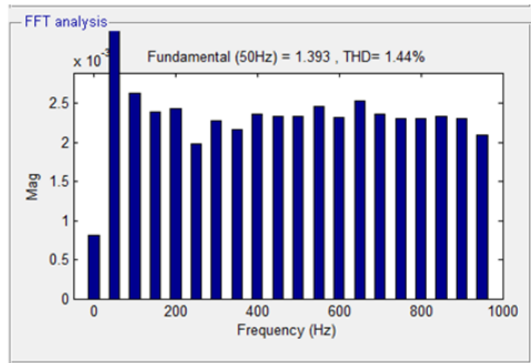
Figure 17. Voltage THD Value of Swell from wind source after compensation.
