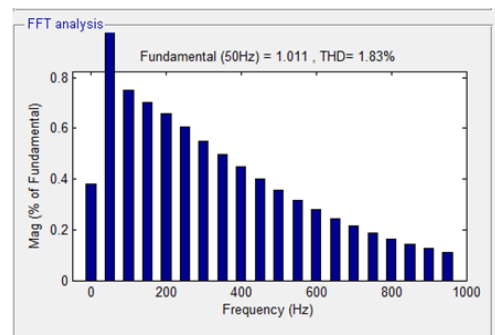
Figure 31. Voltage THD Value of Swell from wind source after compensation.
