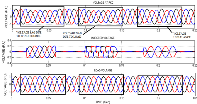
Figure 22. PCC Voltage with sag, unbalance and harmonics, injected voltage, load voltage.
